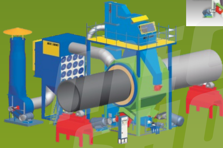
Airless 2W Special Huge Dia Pipe Cleaning M/c
