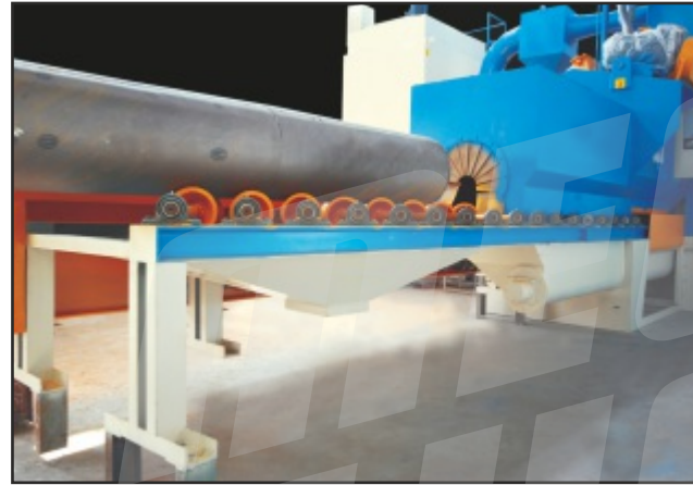
Airless 2 Wheel Diabola Type Shot Blasting M/c for Pipe Cleaning
